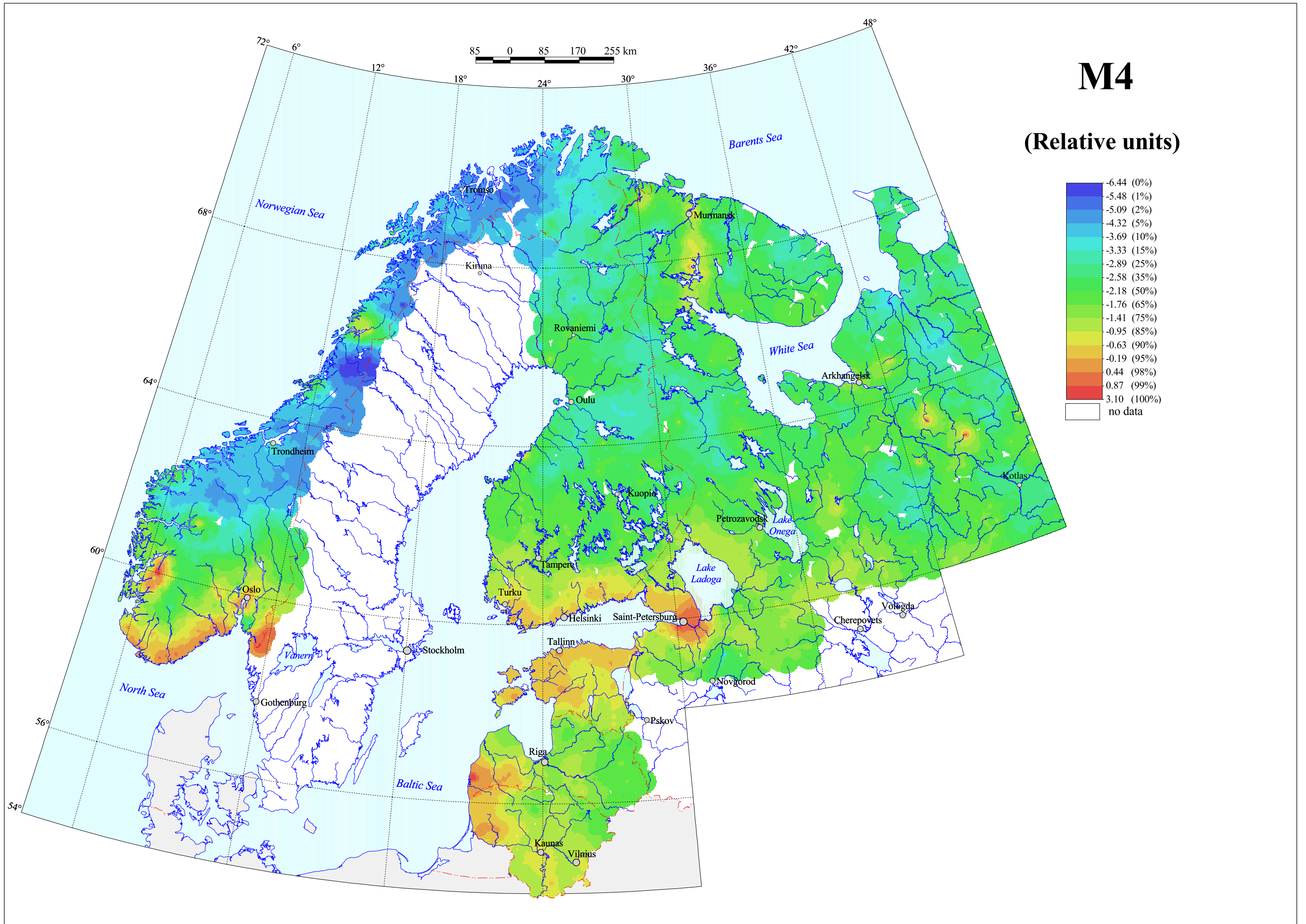
M4 (Cd, Sb, Mo, Pb, Sn, Zn) in Terrestrial Moss, Total Content
